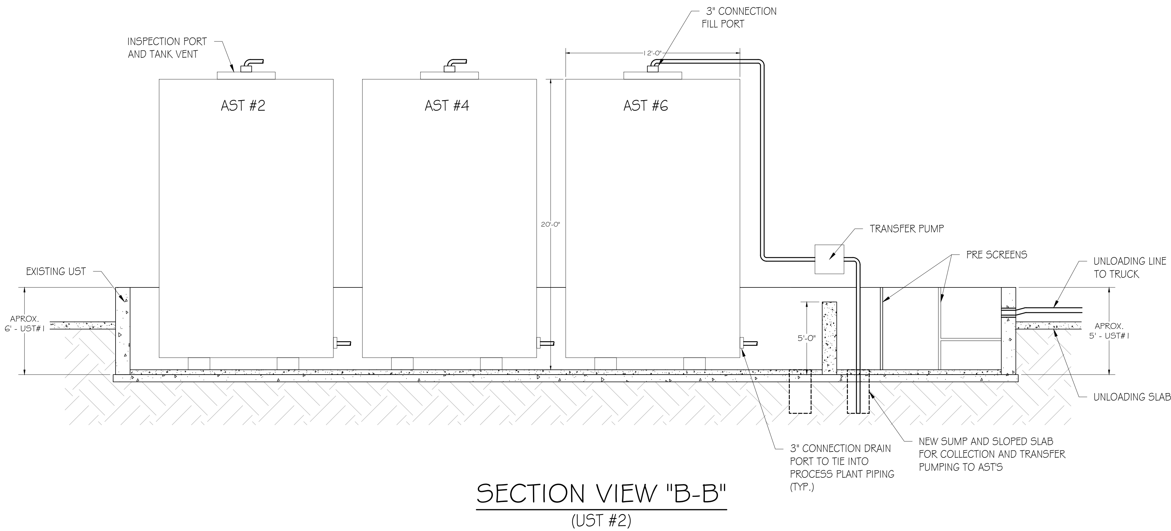
FIGURE 9 UST RETROFIT SECTIONS SCALE: 1/4" = 1'-0"
