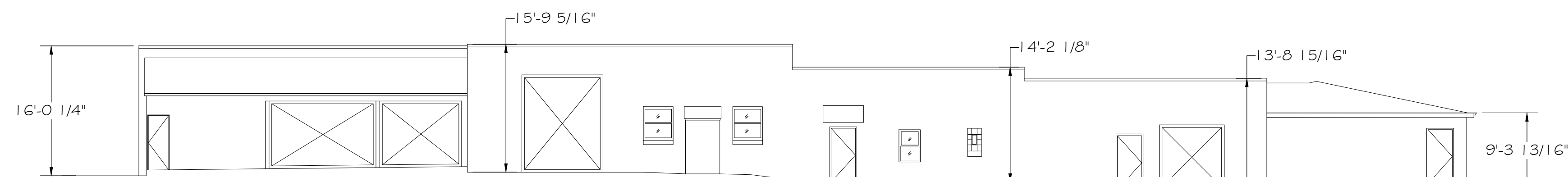
NORTH ELEVATION
