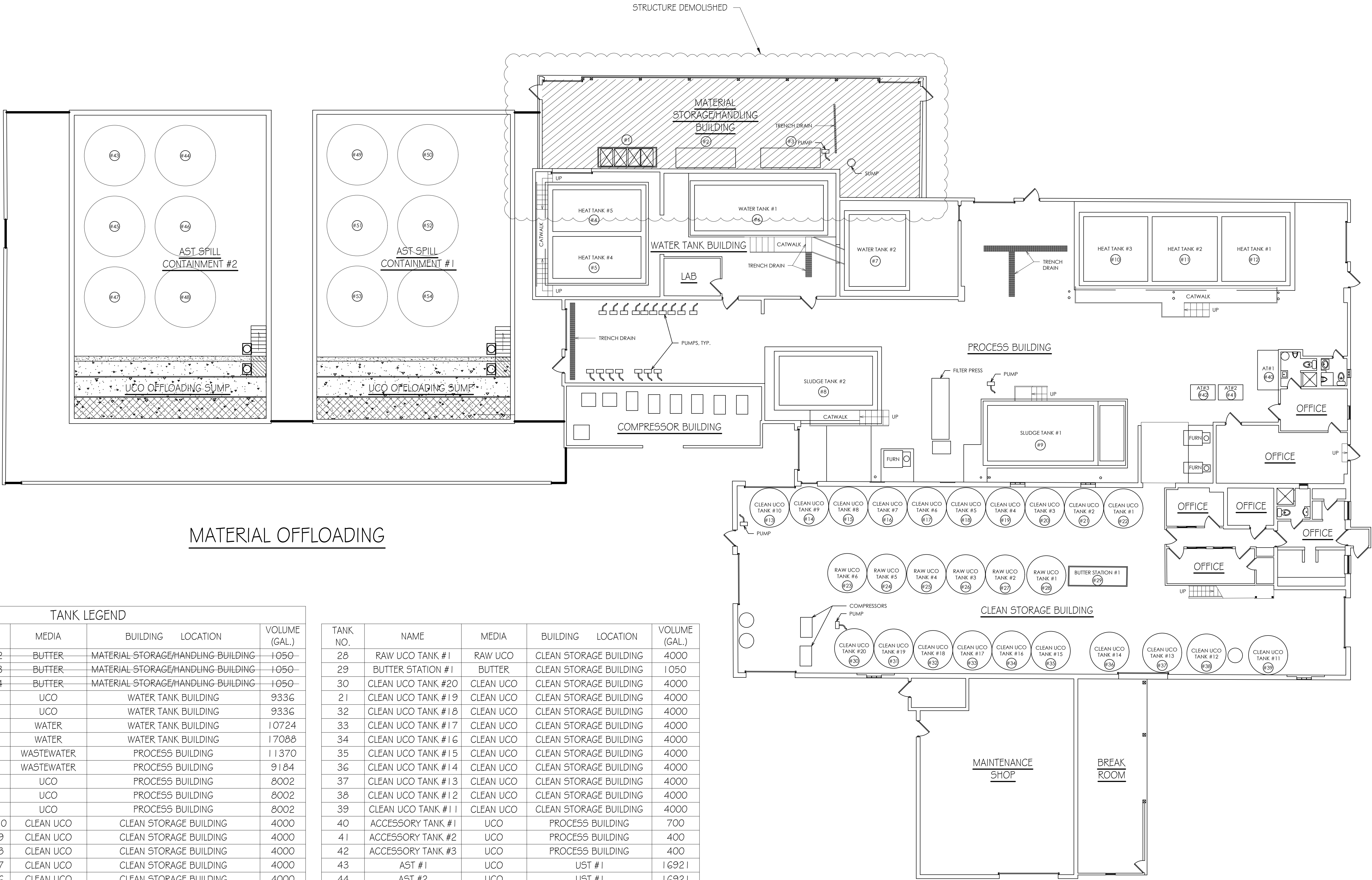
FIGURE 6A PROPOSED TANK LAYOUT PLAN SCALE: NTS
