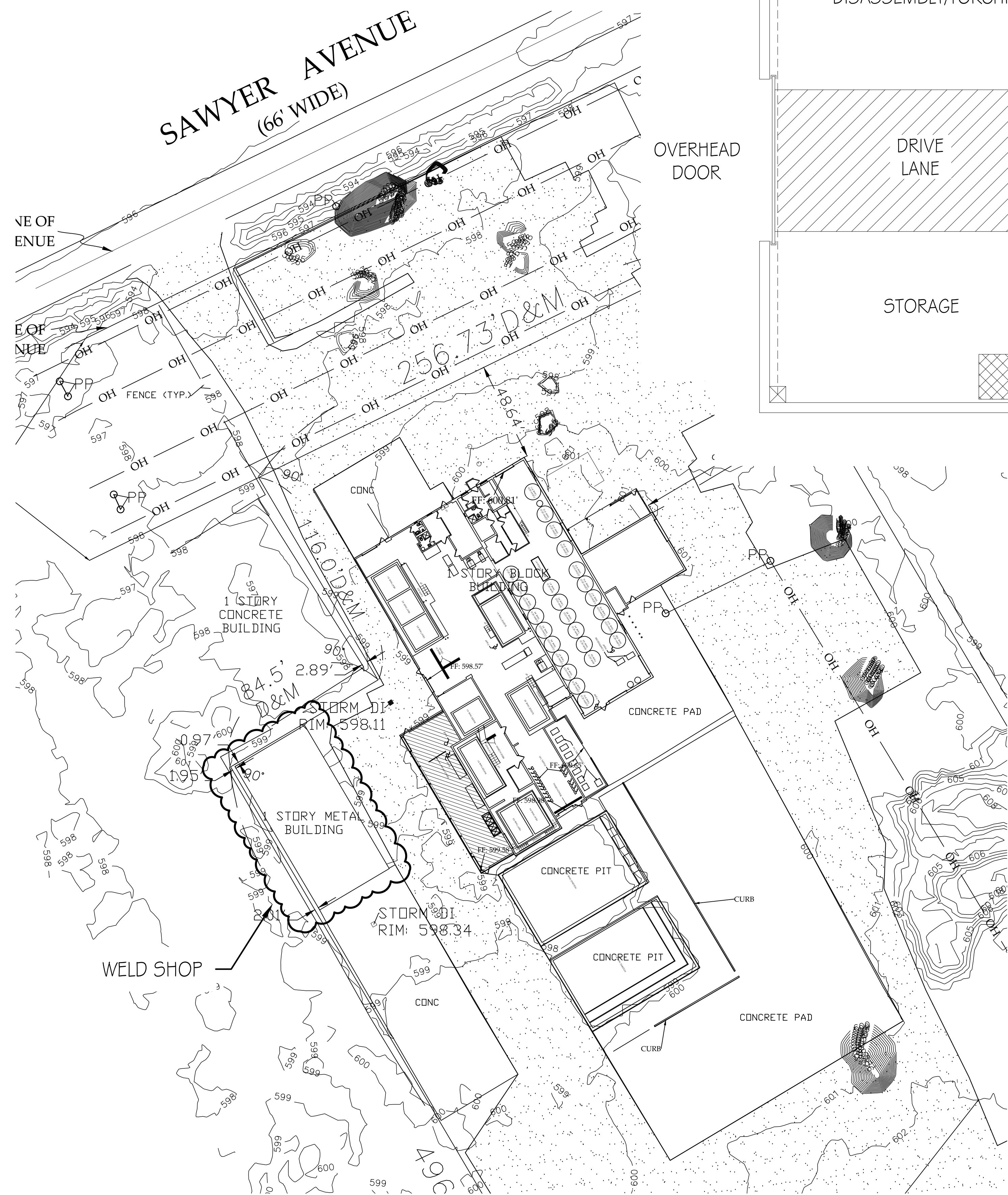
FIGURE 13 WELD SHOP LAYOUT PLAN SCALE: NTS
