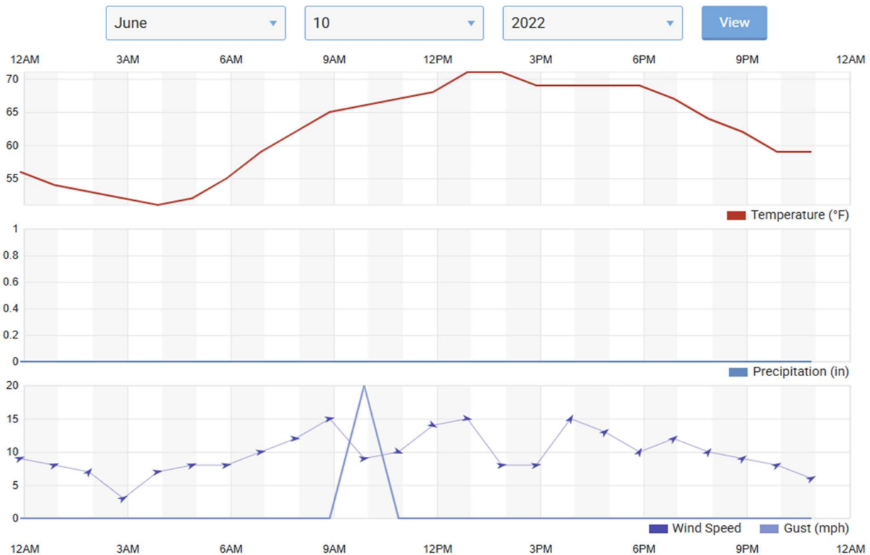
Figure 5. Daily Summary of Meteorological Conditions During Noise Survey (June 10, 2022)
