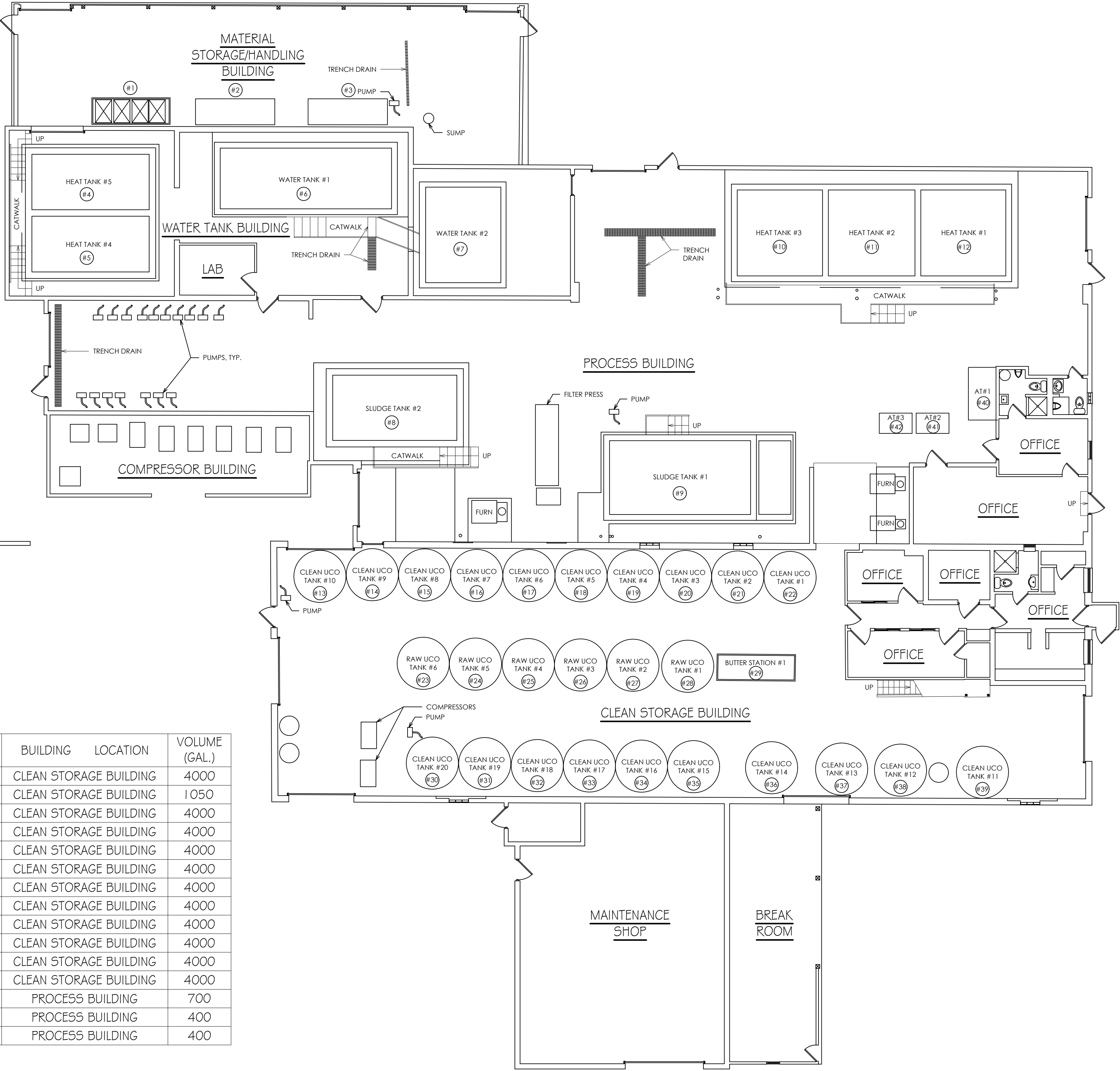
FIGURE 6 EXISTING TANK LAYOUT PLAN SCALE: NTS
