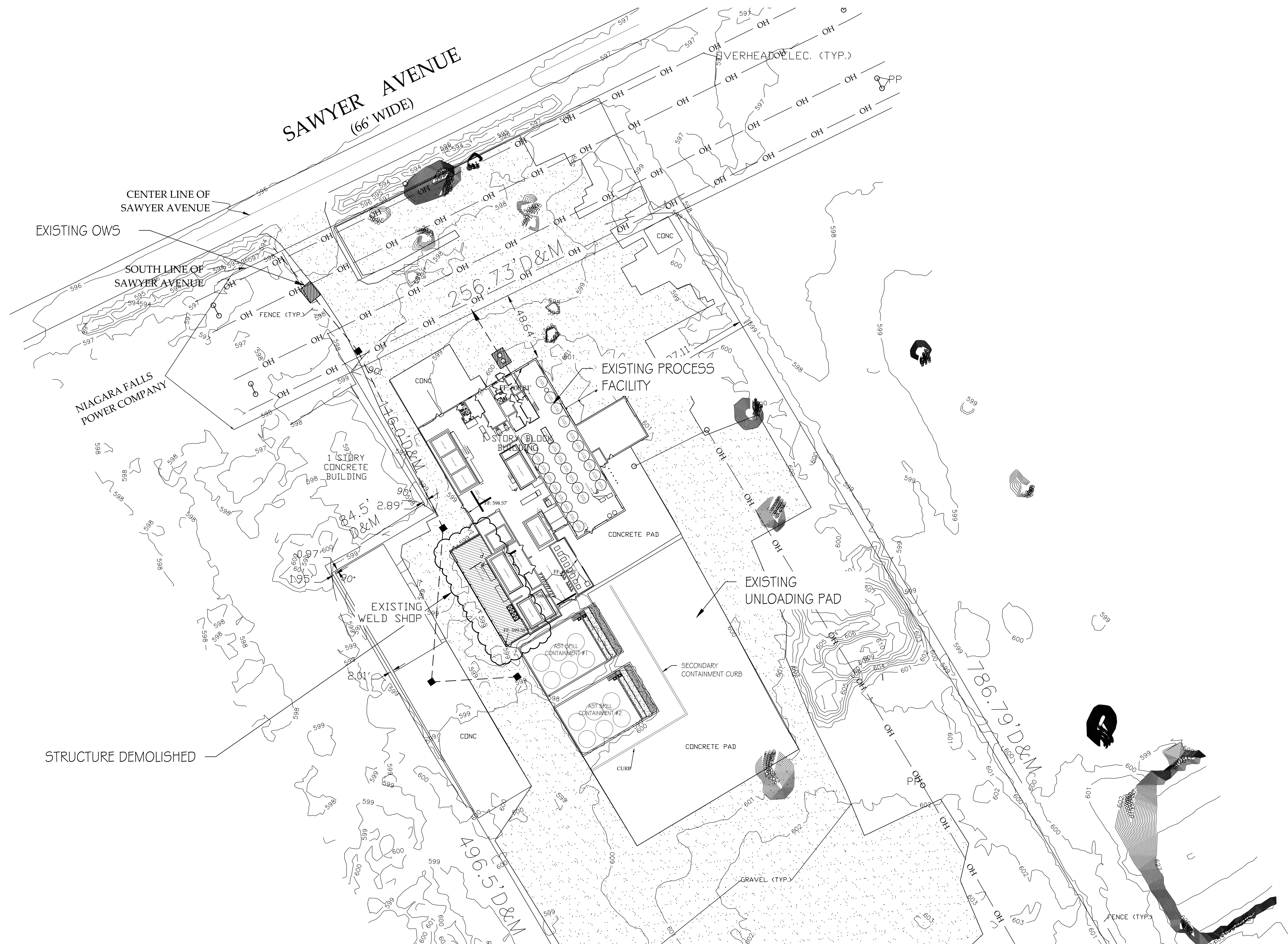
FIGURE 2A PROPOSED SITE PLAN SCALE: NTS
