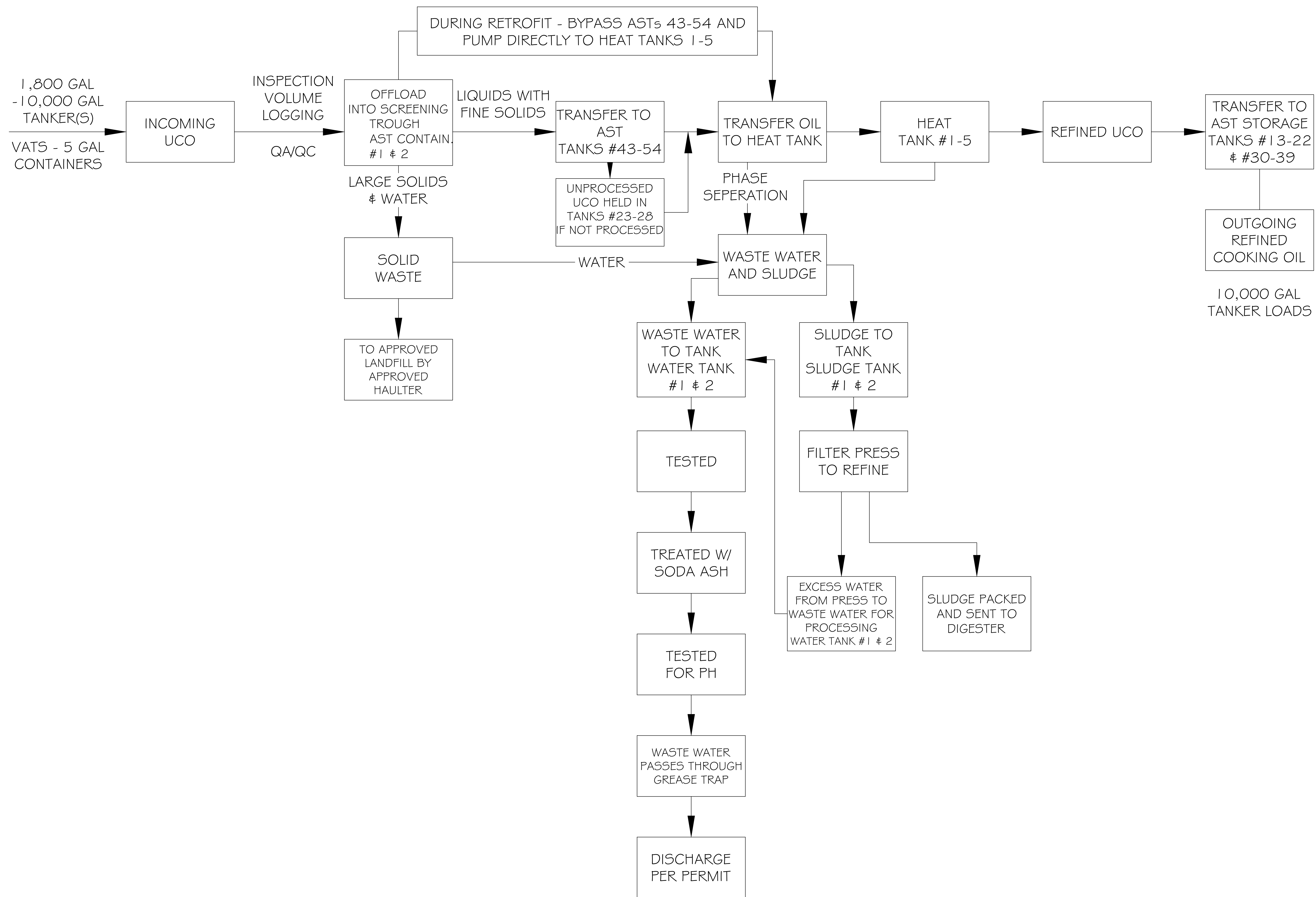
FIGURE 5 PROCESS FLOW
