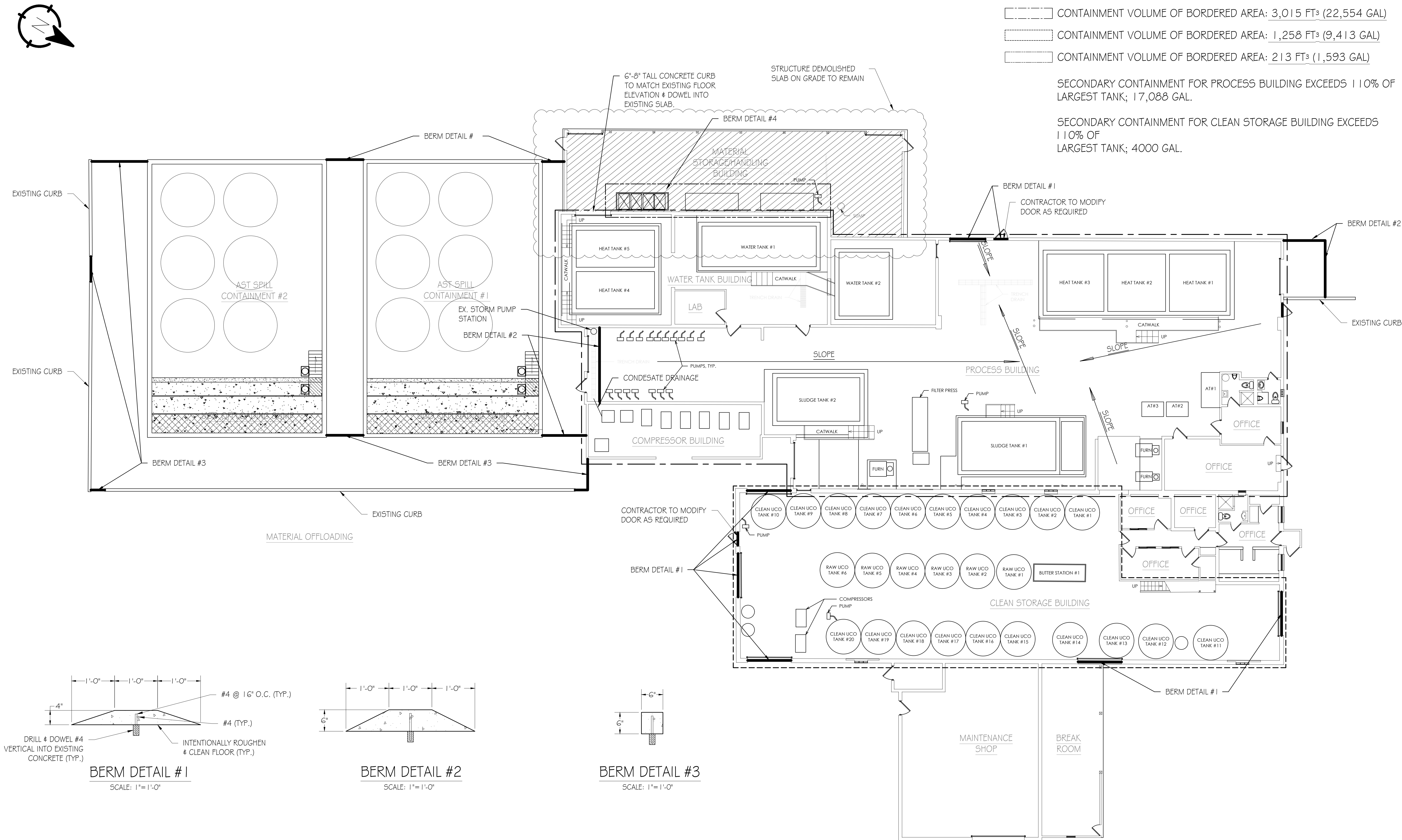
FIGURE 10 SECONDARY SPILL CONTAINMENT PLAN SCALE: NTS
