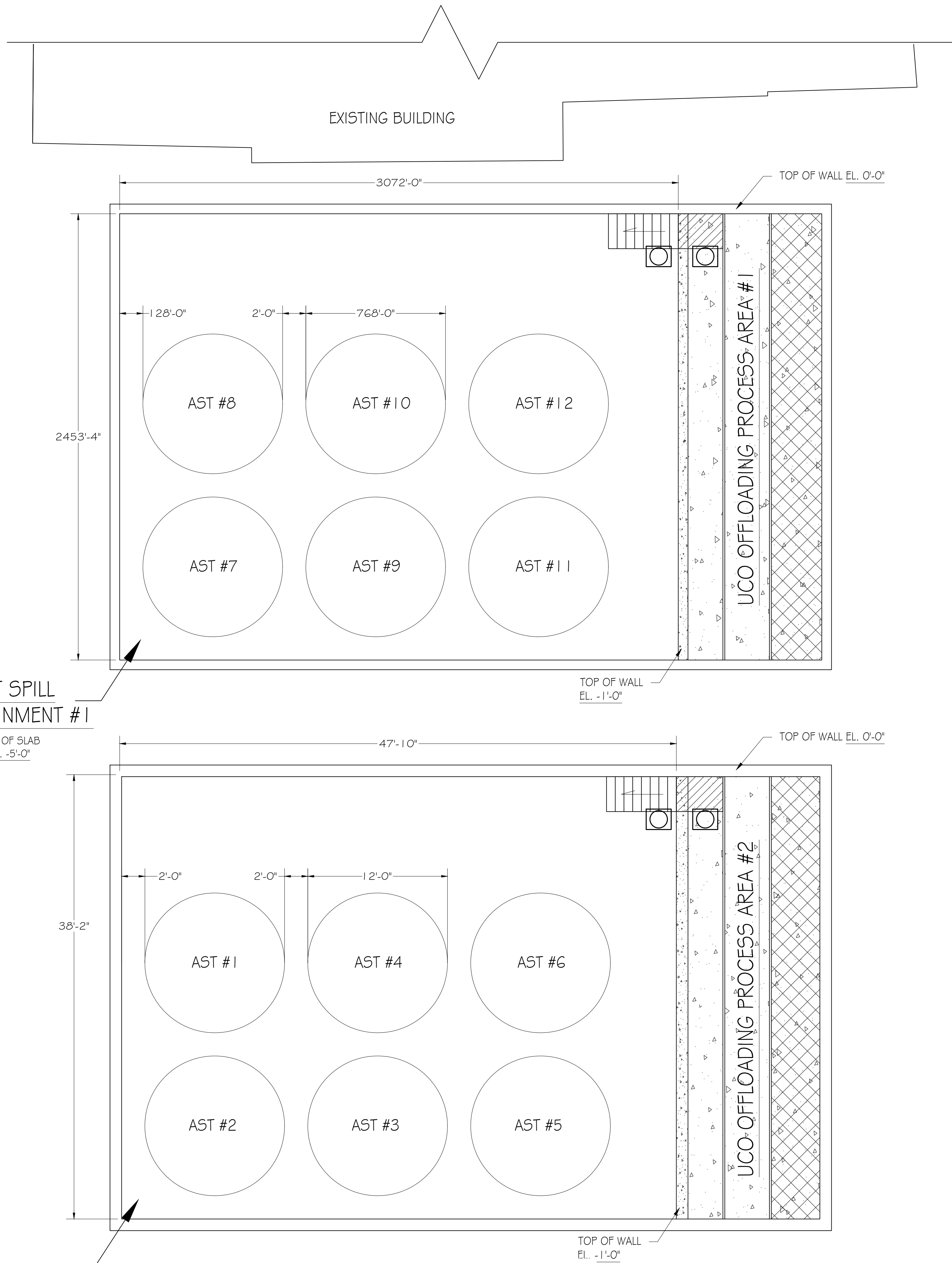
FIGURE 7 NEW AST LAYOUT PLAN SCALE: 3/16"=1'-0"
