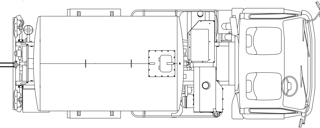
FIGURE 8 LOADING-UNLOADING PLAN SCALE: 3/16" = 1'-0"
